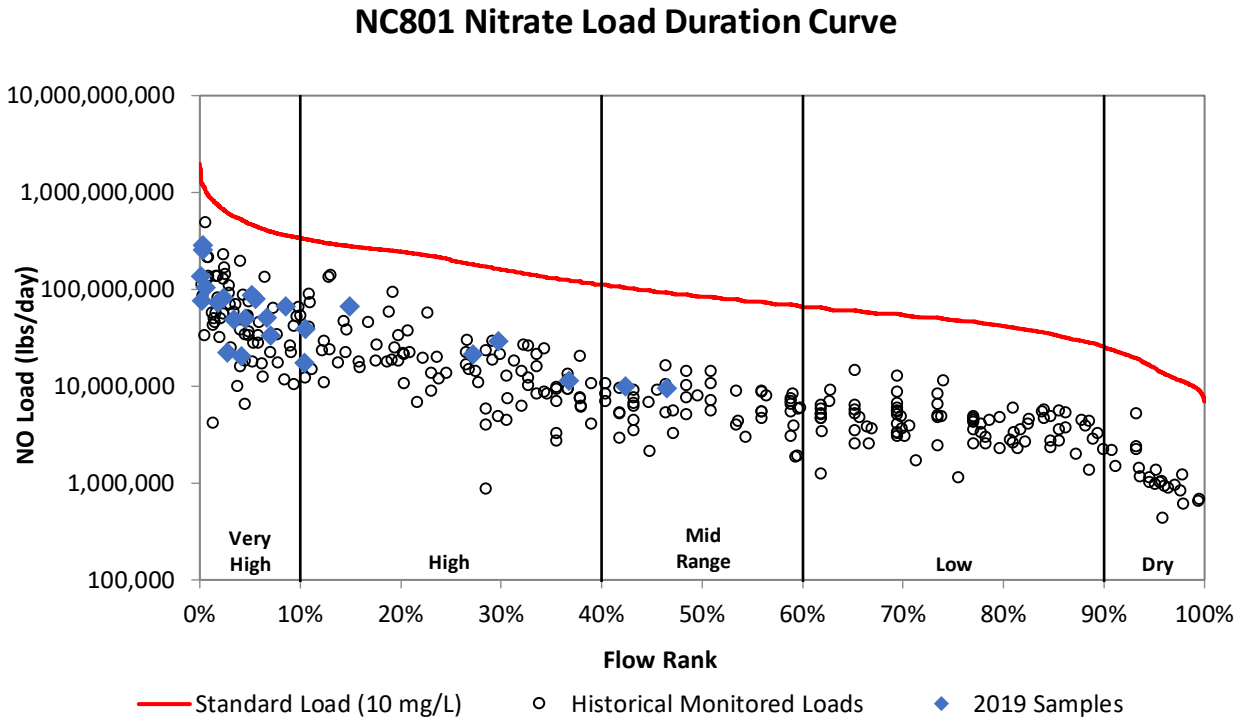
Figure 24f. Load duration curve for nitrate at NC801.
