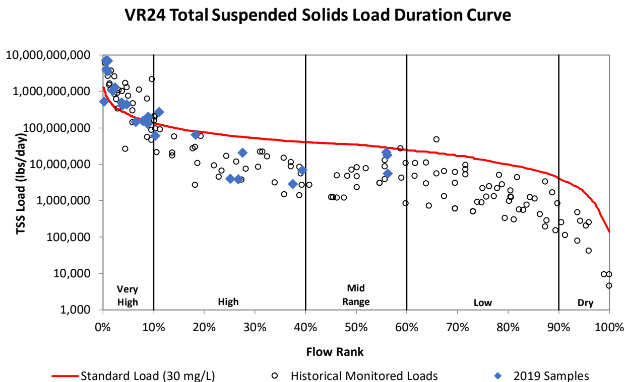
Figure 26a. Load duration curve for total suspended solids at VR24.
