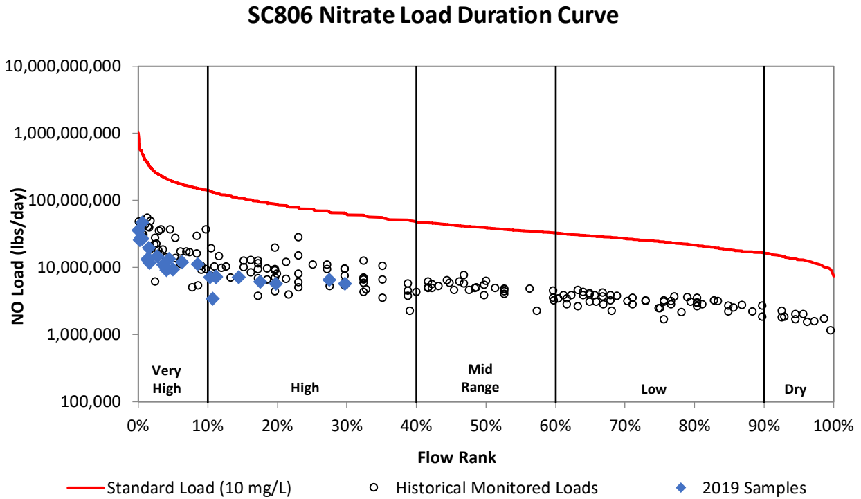
Figure 24b. Load duration curve for nitrate at SC806.
