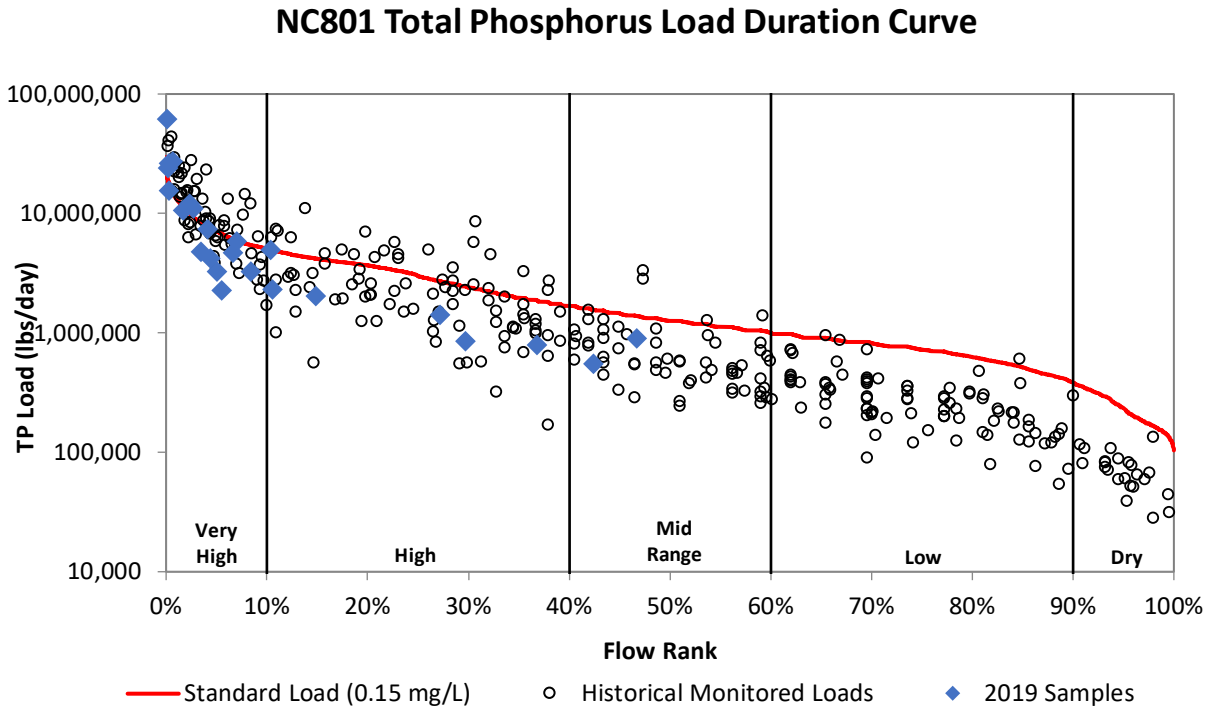
Figure 25f. Load duration curve for total phosphorus at NC801.
