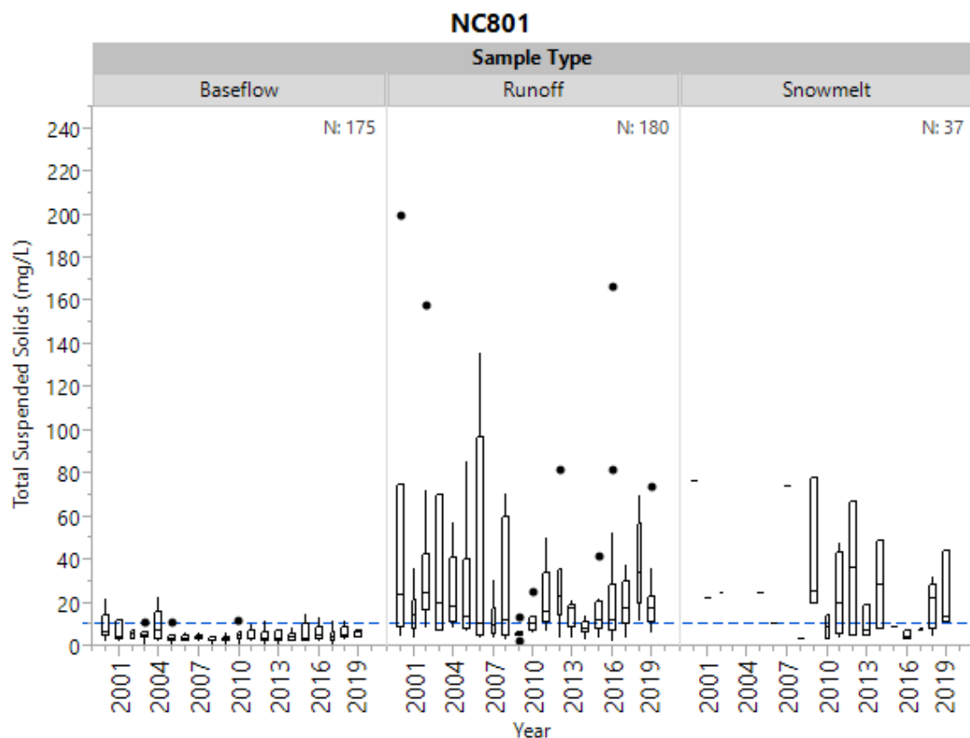
Figure 20f. Historical total suspended solids by sample type at NC801.
