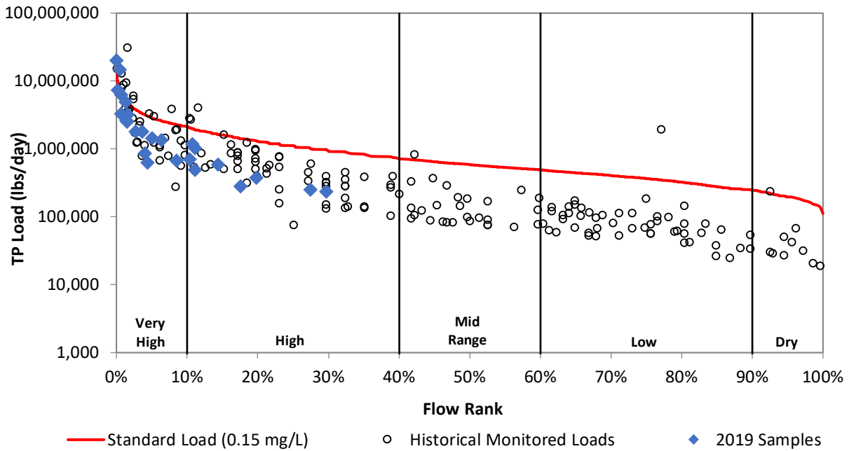
Figure 25b. Load duration curve for total phosphorus at SC806.
