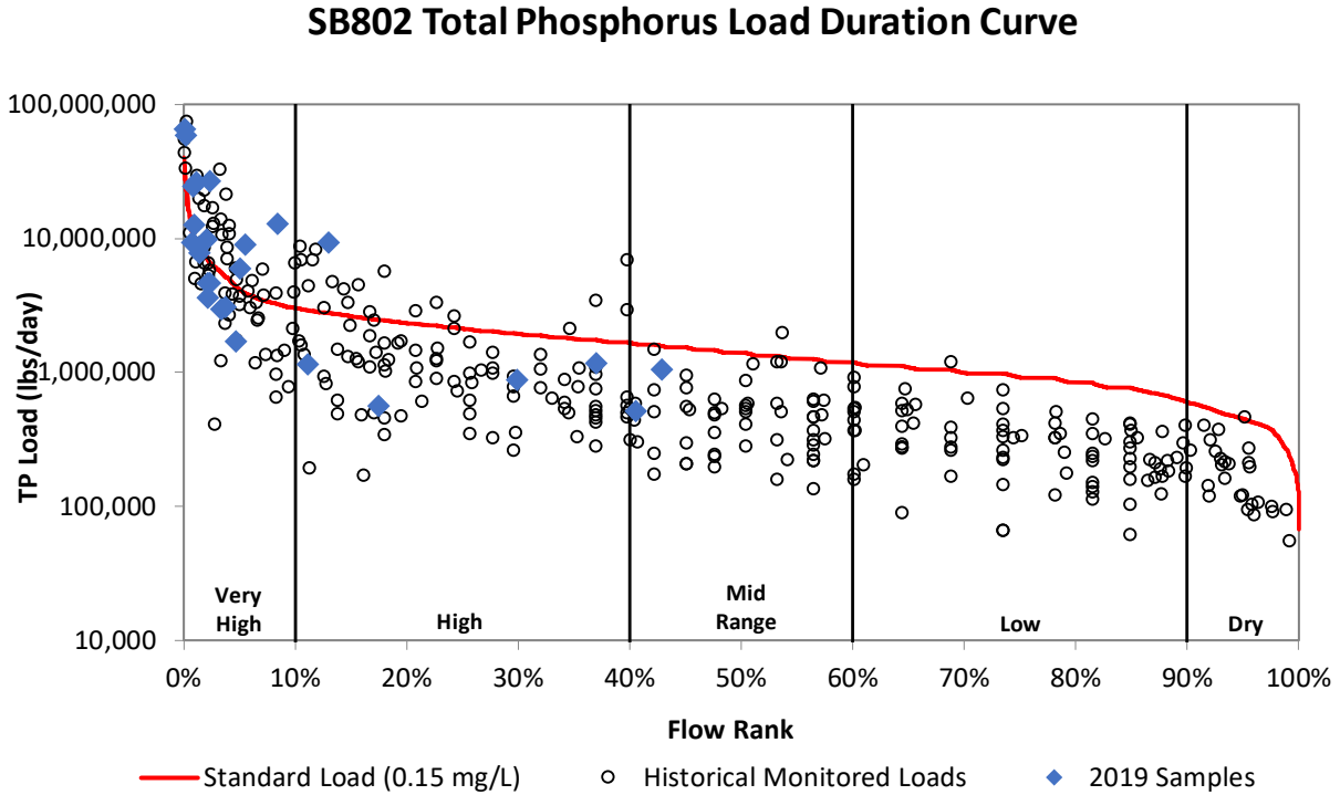
Figure 25g. Load duration curve for total phosphorus at SB802.
