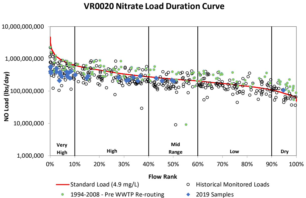
Figure 24i. Load duration curve for nitrate at VR0020.
