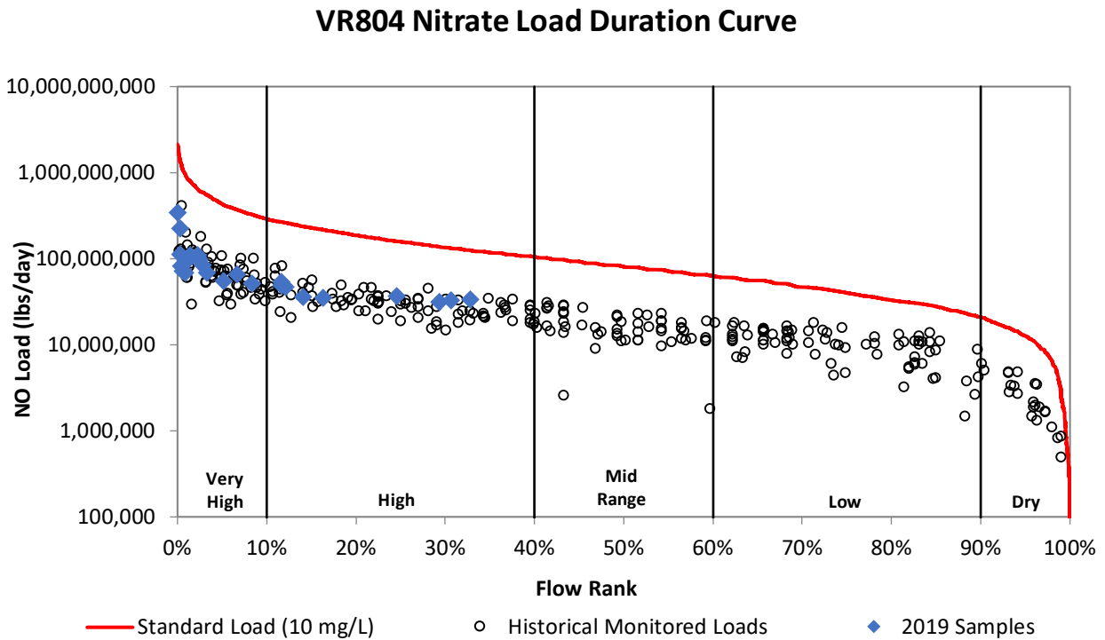
Figure 24c. Load duration curve for nitrate at VR804.
