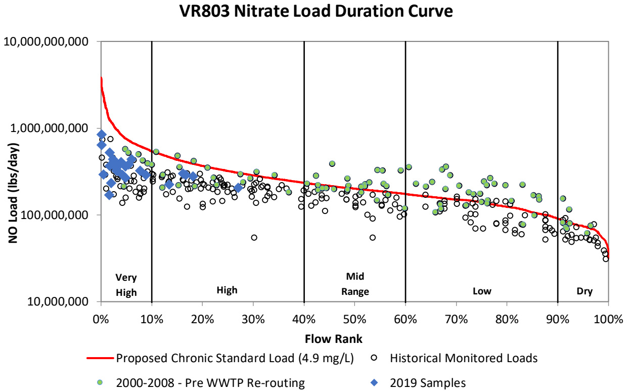
Figure 24h. Load duration curve for nitrate at VR803.
