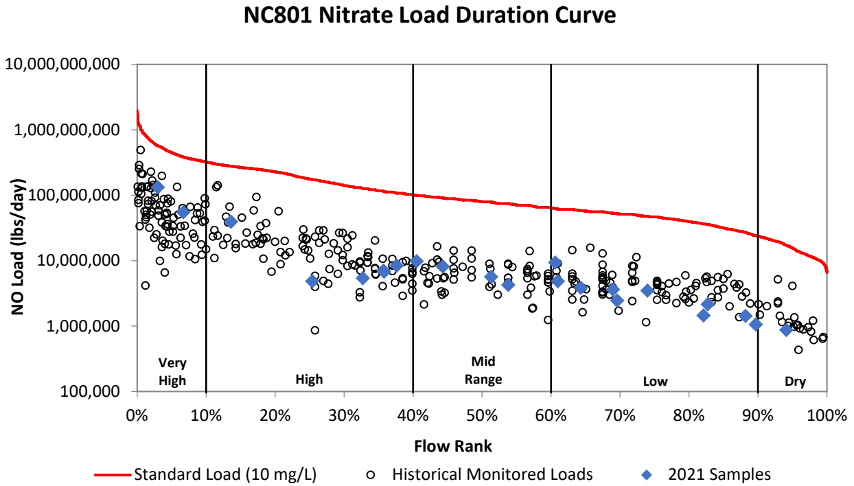
Figure 26f. Load duration curve for nitrate at NC801.
