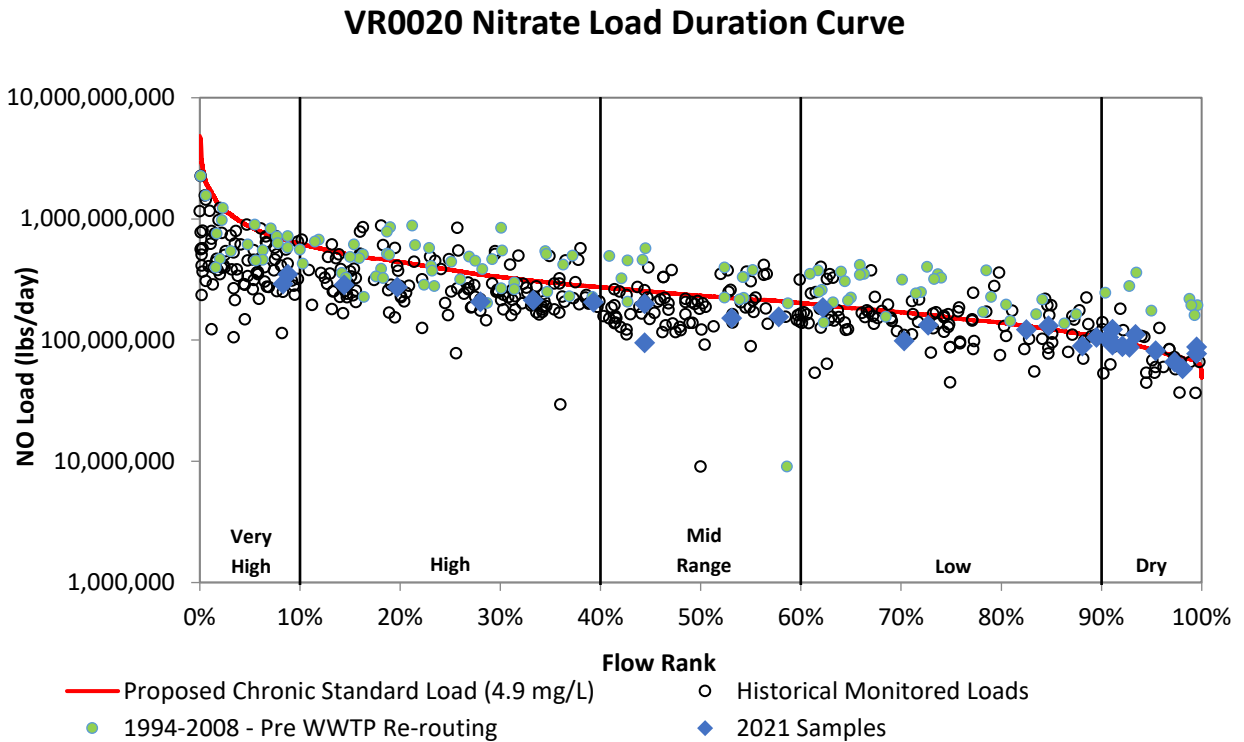
Figure 26i. Load duration curve for nitrate at VR0020.
