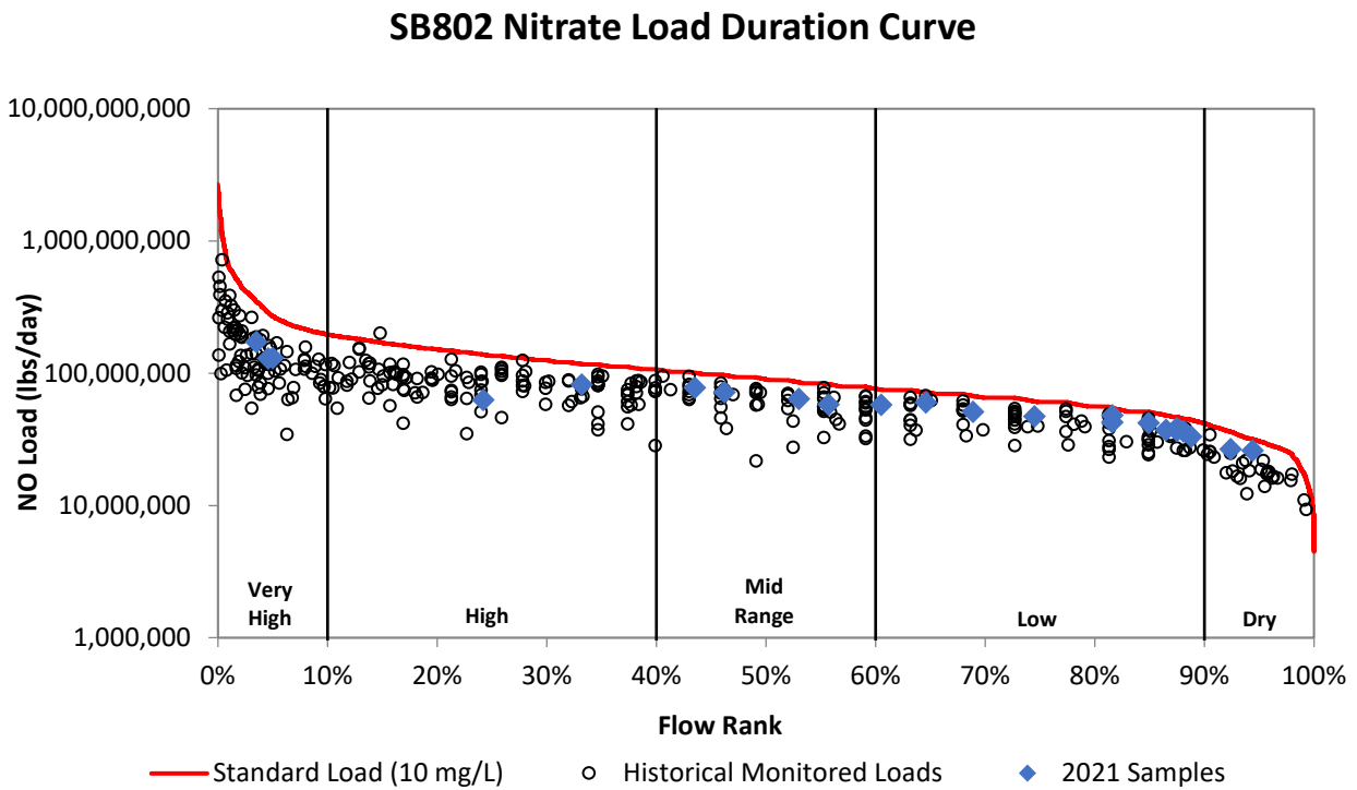
Figure 26g. Load duration curve for nitrate at SB802.
