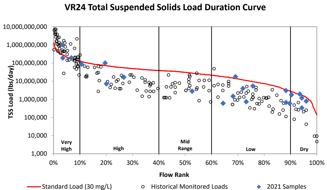
Figure 28a. Load duration curve for total suspended solids at VR24.
