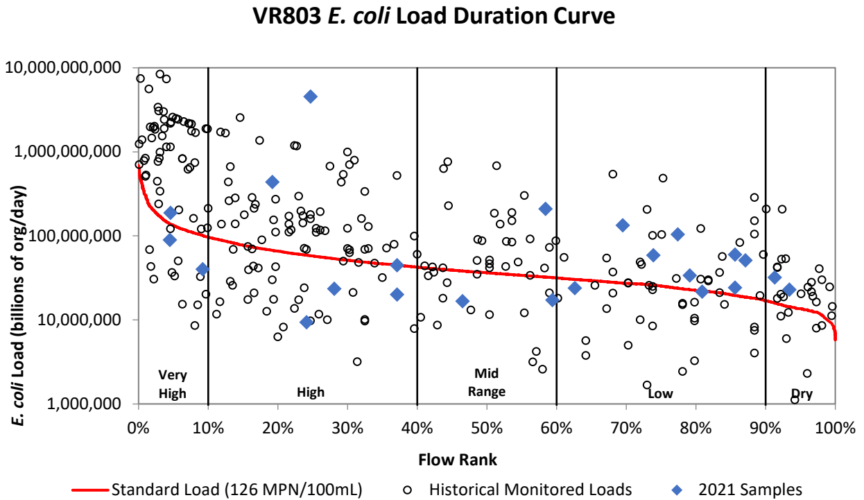
Figure 25h. Load duration curve for E. coli at VR803.
