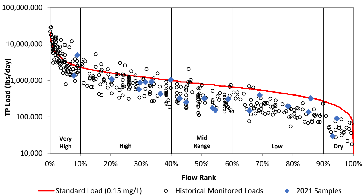
Figure 27e. Load duration curve for total phosphorus at NC808.
