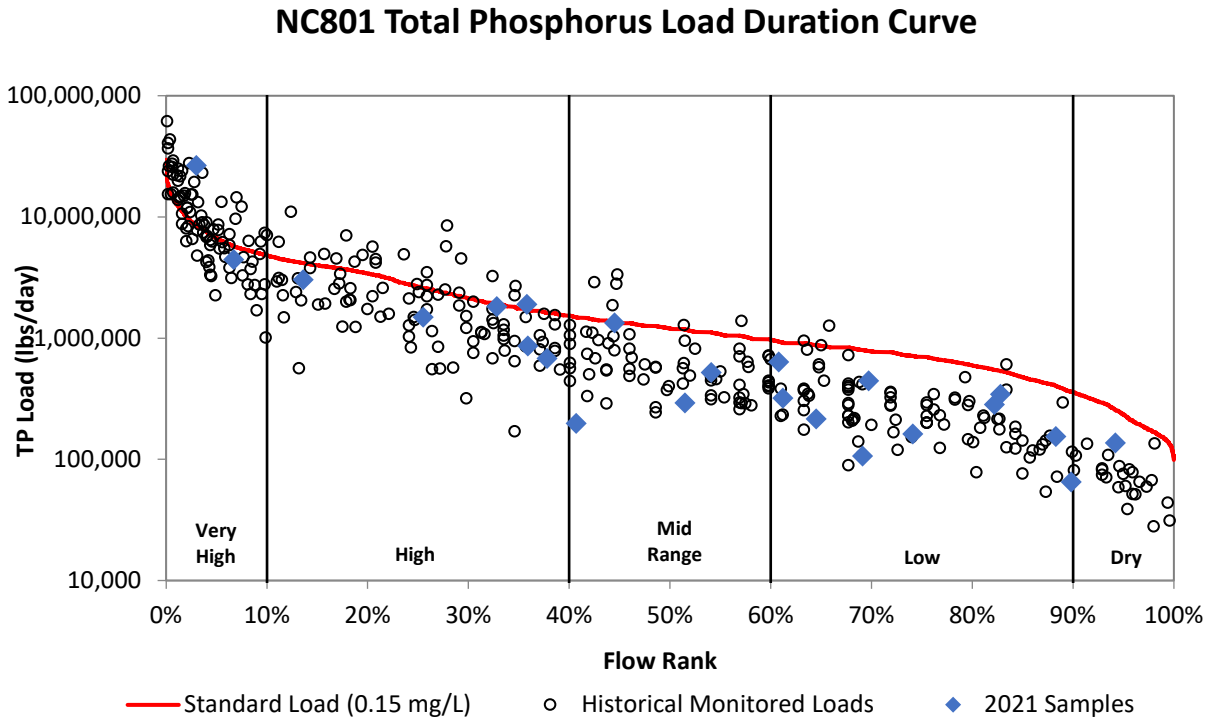
Figure 27f. Load duration curve for total phosphorus at NC801.
