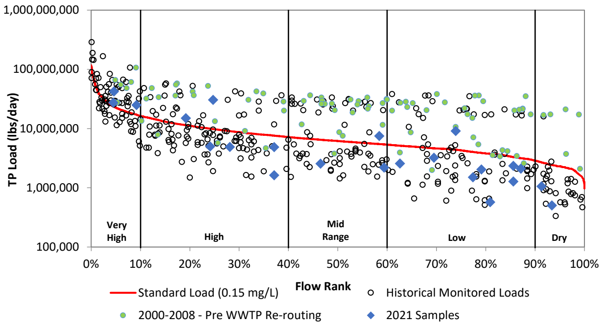
Figure 27h. Load duration curve for total phosphorus at VR803.
