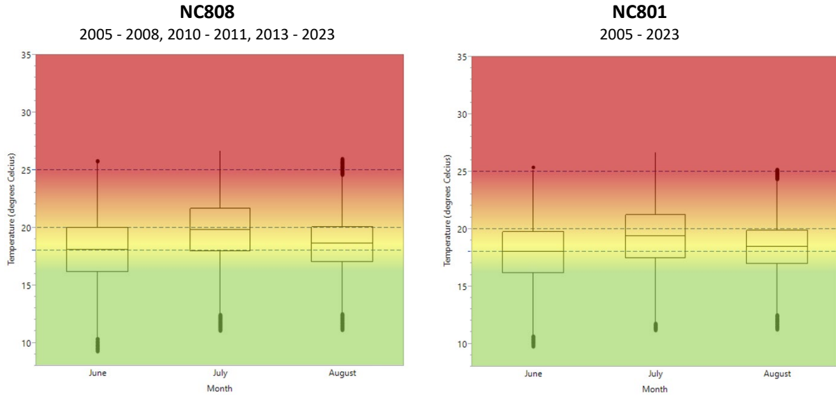
Figure 8. Continuous temperature data for NC808 and NC801 (coldwater stream sites) during the summer months from 2005-2023 (when available). Temperature ranges apply to adult Brown Trout. Optimal <18°C, tolerance 18-20°C, resistance 20-22°C, and complete mortality at 25°C (Coutant (1975), Gardner & Leetham (1914), Bell (2006))
