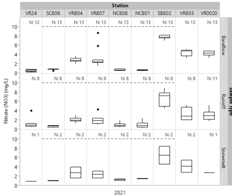
Figure 2. Nitrate nitrogen for each station, categorized by sample type, for 2021. Blue dashed line represents the domestic consumption state standard ( \leq 10 mg/L).
