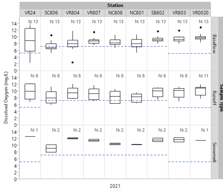
Figure 4. Dissolved oxygen for each station, categorized by sample type, for 2021. Dashed blue lines indicate standards with 7.0 mg/L (2A streams) and 5.0 mg/L (2B streams) as acceptable daily minimums.
