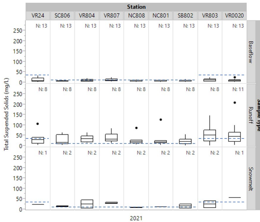
Figure 5. Total suspended solids categorized by sample type for 2021. Blue dashed line represents the state standard for cold 2A ( \leq 10 mg/L) and warm 2B ( \leq 30 mg/L) waters.
