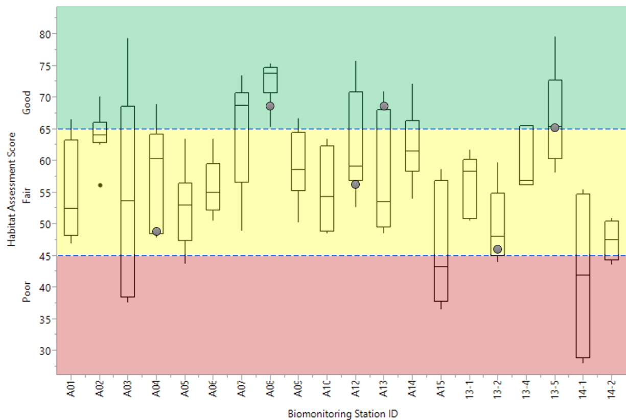
Figure 7. Habitat assessment scores for biomonitoring stations. Habitat scores for 2021 are indicated by grey circle. Dashed blue lines indicate limits for Good ( \geq 66 ), Fair (45-65), and Poor ( \leq 44 ) categories. Number of samples collected from 2009-2021 is shown in parenthesis.
