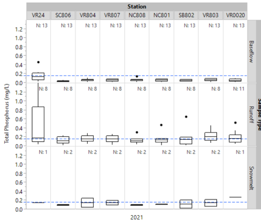
Figure 3. Total phosphorus (TP) for each station, categorized by sample type, for 2021. Blue dashed line represents the state standard for total phosphorus, \leq 0.15 mg/L.
