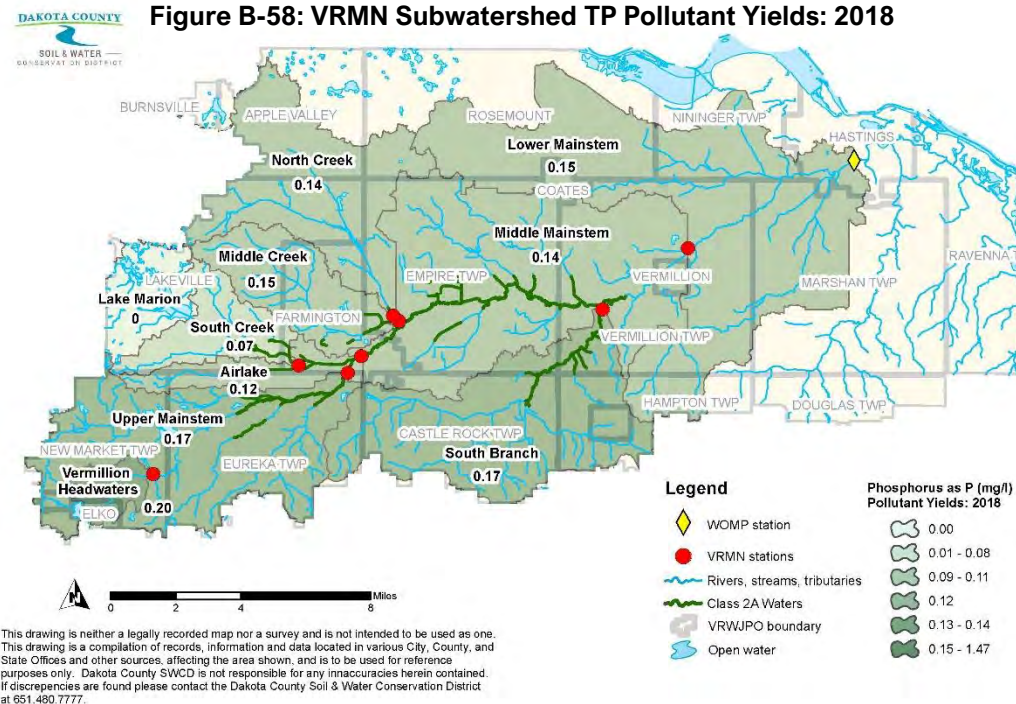
Figure B-58: VRMN Subwatershed TP Pollutant Yields: 2018
