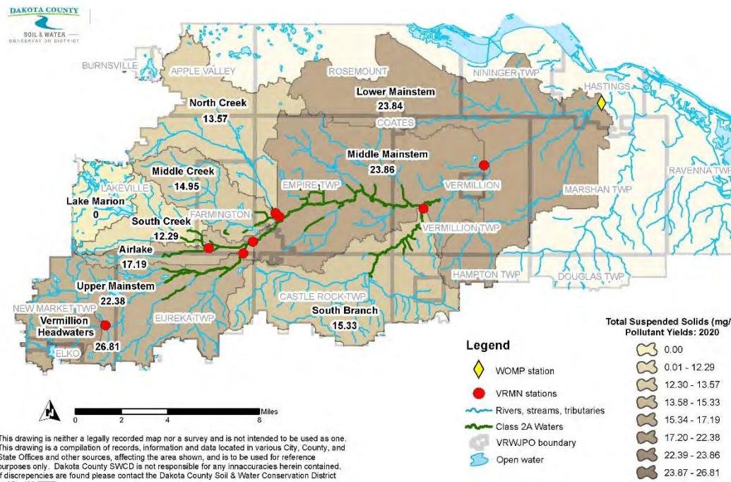
Figure B-51: VRMN Subwatershed TSS Pollutant Yields: 2020
