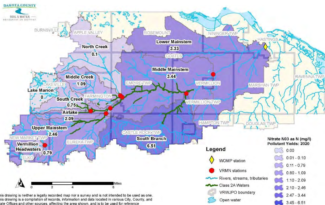
Figure B-69: VRMN Subwatershed Nitrate Pollutant Yields: 2020
