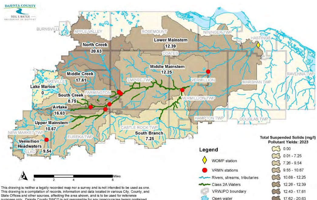
Figure B-54: VRMN Subwatershed TSS Pollutant Yields: 2023
