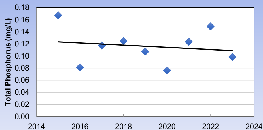
Figure B-91: Lake Rebecca Total Phosphorus
