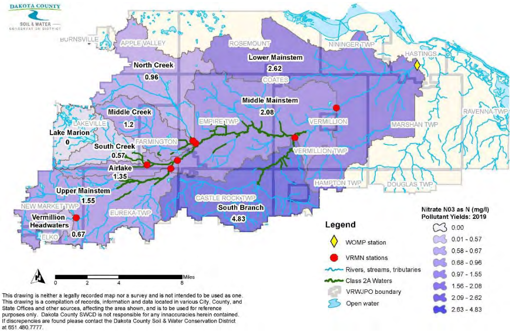
Figure B-68: VRMN Subwatershed Nitrate Pollutant Yields: 2019
