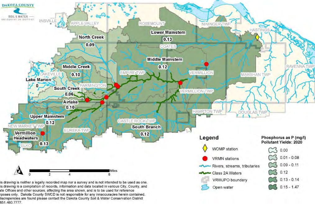
Figure B-60: VRMN Subwatershed TP Pollutant Yields: 2020
