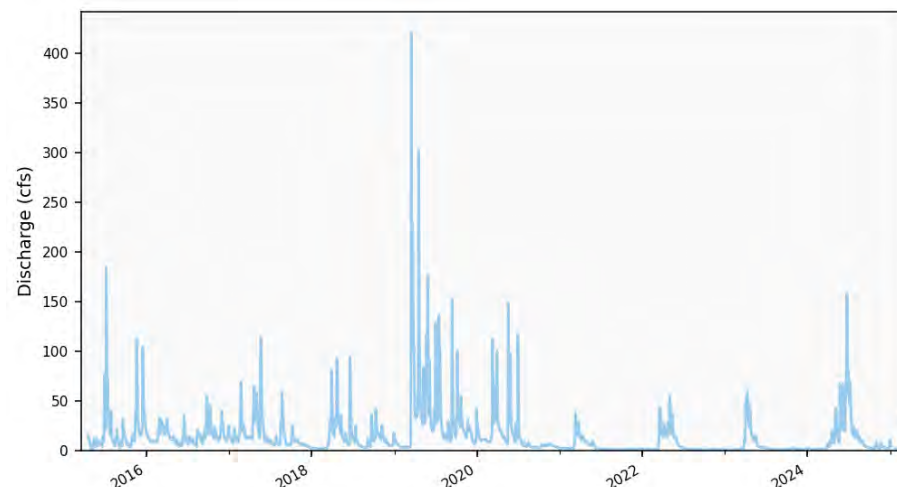
Figure B-76: Vermillion River at Lakeville Stream Discharge: 2015-2025
