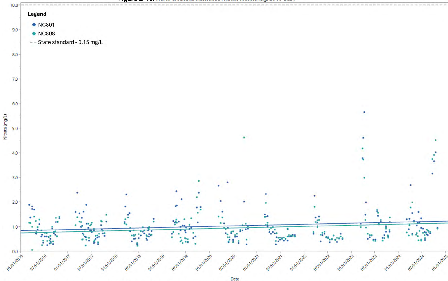
Figure B-40: North Creek Subwatershed Nitrate Monitoring: 2016-2024
