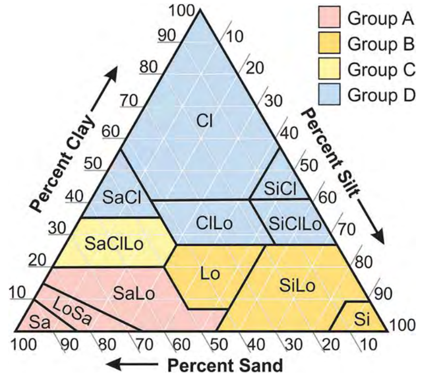
Figure B-15: Soil Texture Triangle
