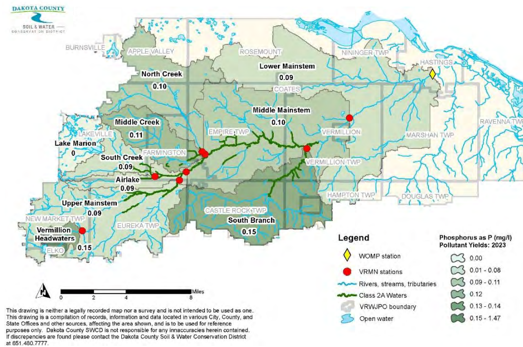
Figure B-63: VRMN Subwatershed TP Pollutant Yields: 2023
