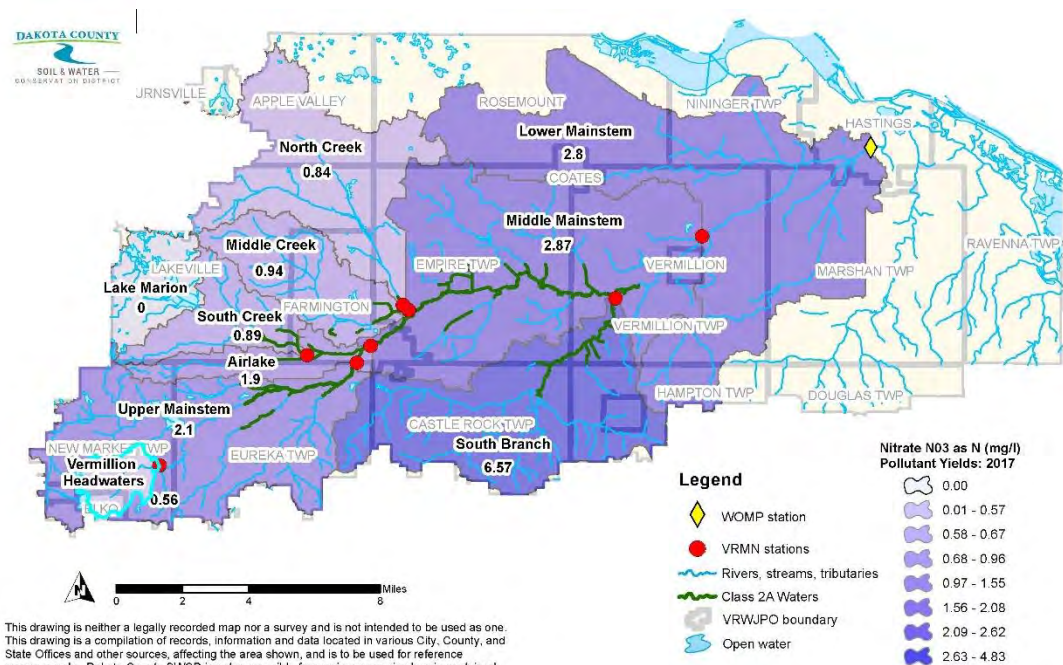
Figure B-66: VRMN Subwatershed Nitrate Pollutant Yields: 2017
