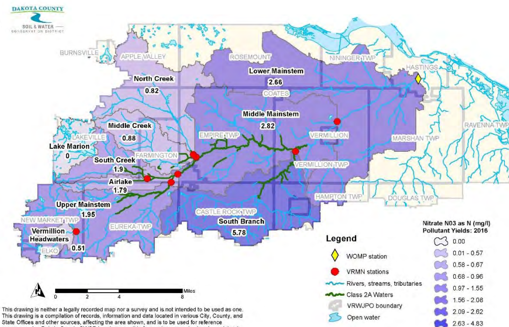
Figure B-65: VRMN Subwatershed Nitrate Pollutant Yields: 2016
