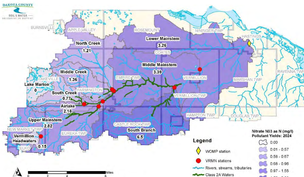
Figure B-73: VRMN Subwatershed Nitrate Pollutant Yields: 2024
